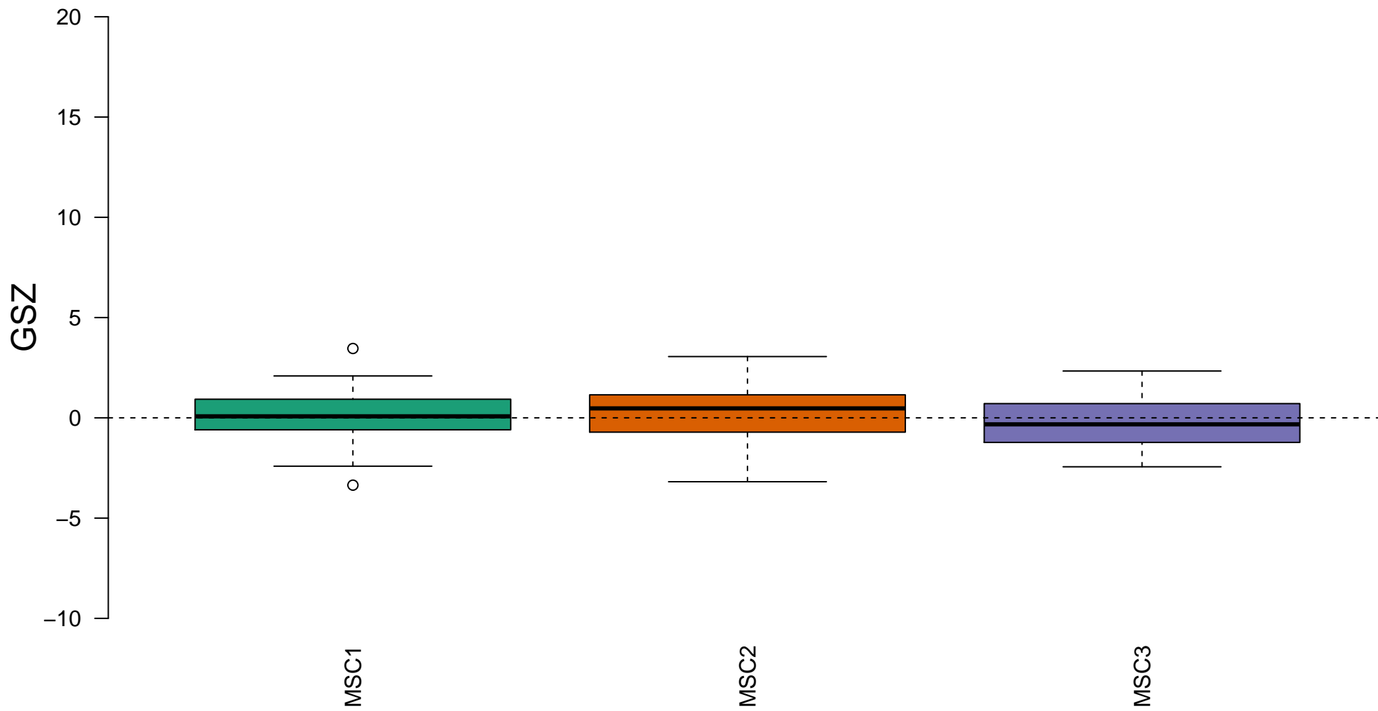
maturation of SSU-rRNA from tricistronic rRNA transcript (SSU-rRNA, 5.8S rRNA, LSU-rRNA)
